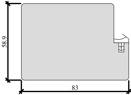
Blockrahmen Standard
